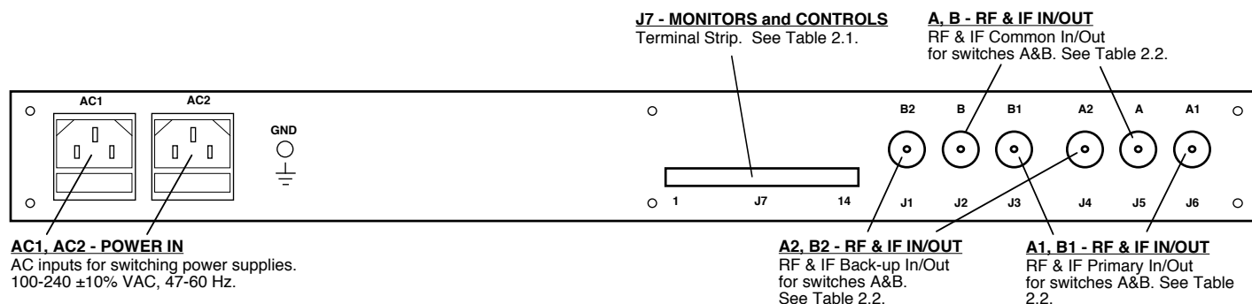
FIGURE 2.2 1582-71/72 RF Switch Rear Panel Inputs/Outputs
