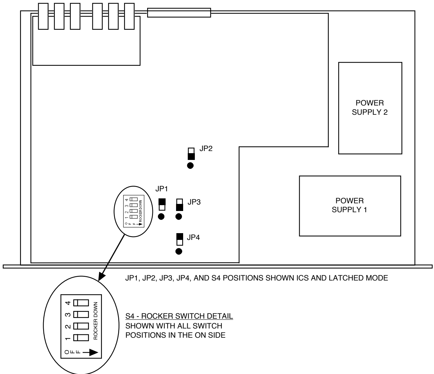
FIGURE 2.1 1582-71/72 RF Switch Assembly
