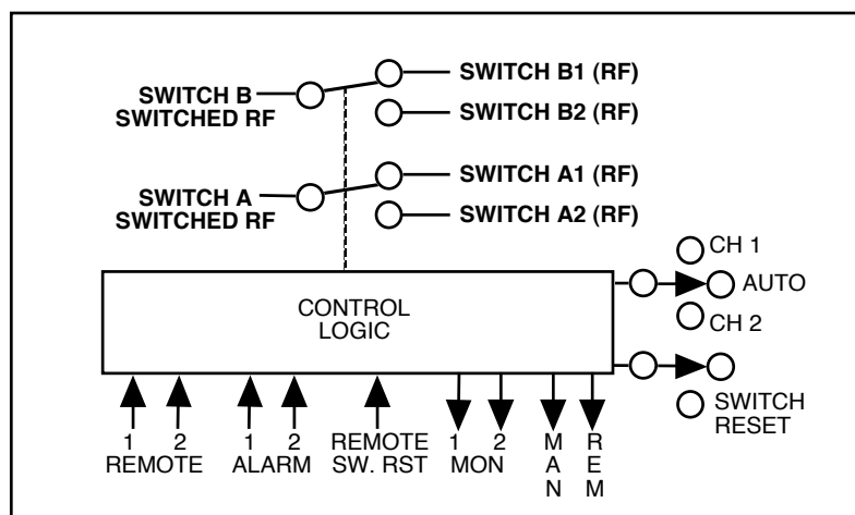
FIGURE 1.2 Model 1582-71/72 RF Switch Block Diagrams
