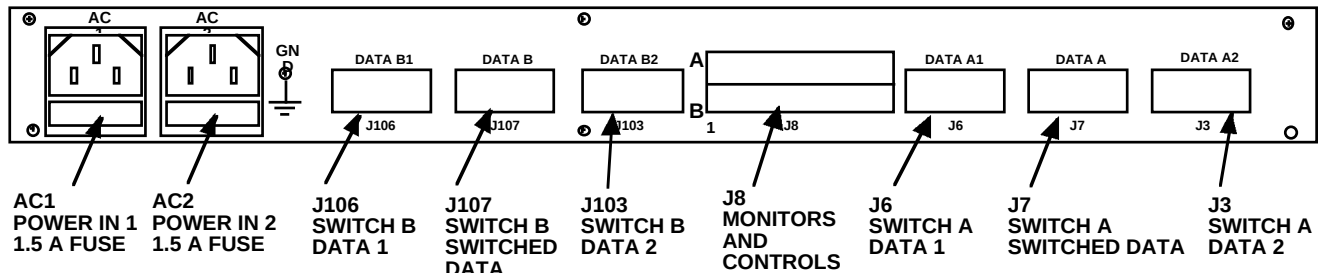
FIGURE 2.0 1582-04 Rear Panel I/O's
