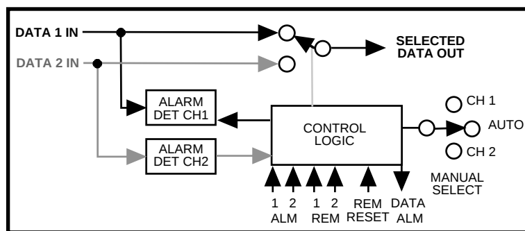
FIGURE 1.2 Model 1582-04 Data Switch Block Diagram (Each Switch)
