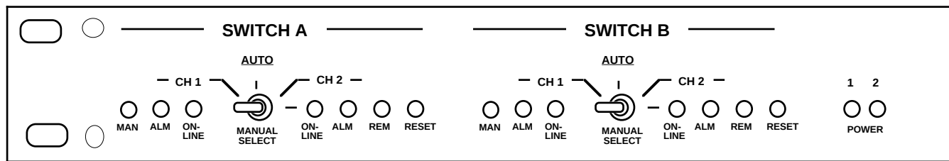
FIGURE 2.2 1582-04 Front Panel Controls and Indicators
