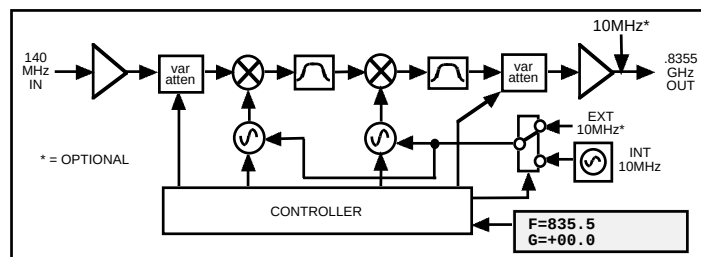
Block Diagram
