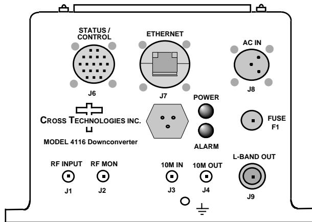
Model 4116-200 Ka-Band Block Downconverter Front Panel
