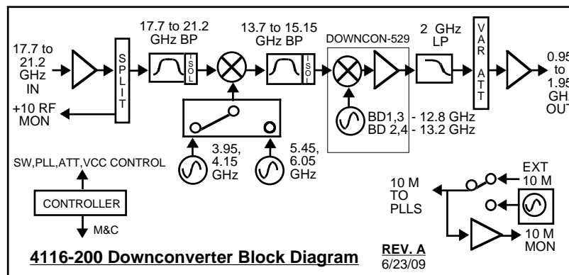
FIGURE 1 Model 4116-200 Ka-Band Block Downconverter Block Diagram
