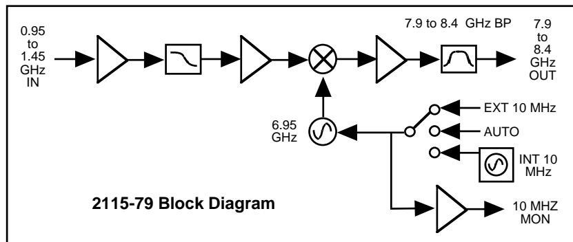
FIGURE 1.2 Block Diagram
