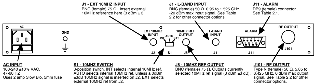
FIGURE 2.1 2115-58 Rear Panel I/O's
