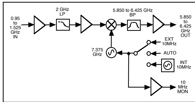
FIGURE 1.2 Model 2115-58 Upconverter Block Diagram
