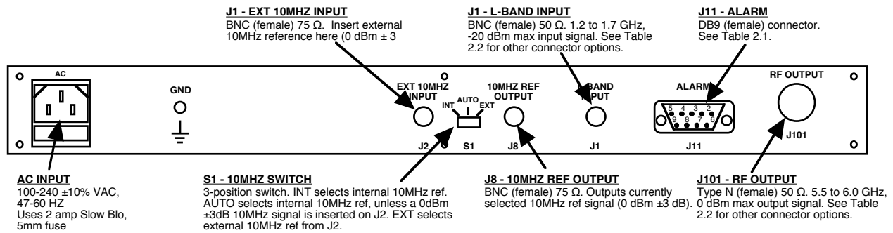
FIGURE 2.1 2115-55 Rear Panel I/O's
