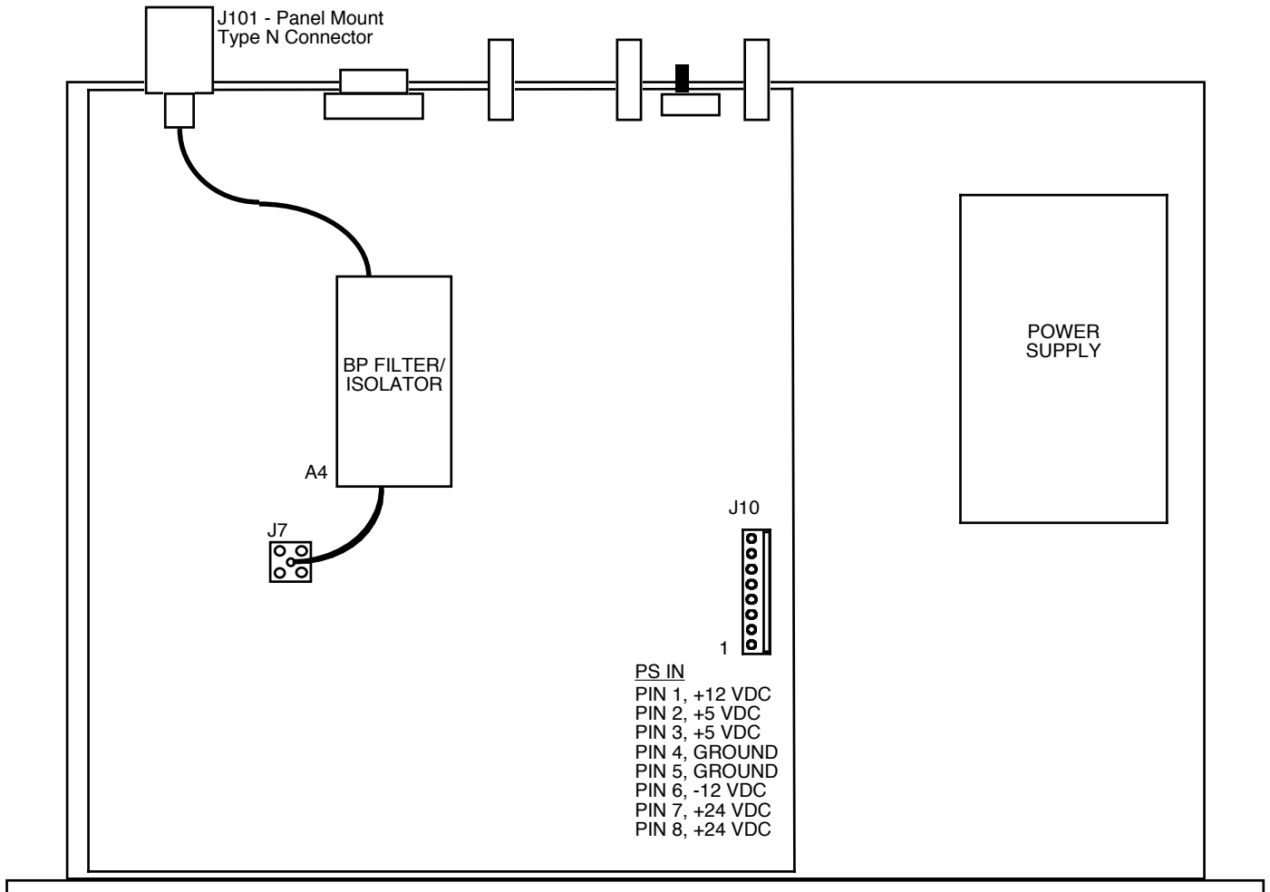
FIGURE 2.0 2115-55 Mechanical Assembly
