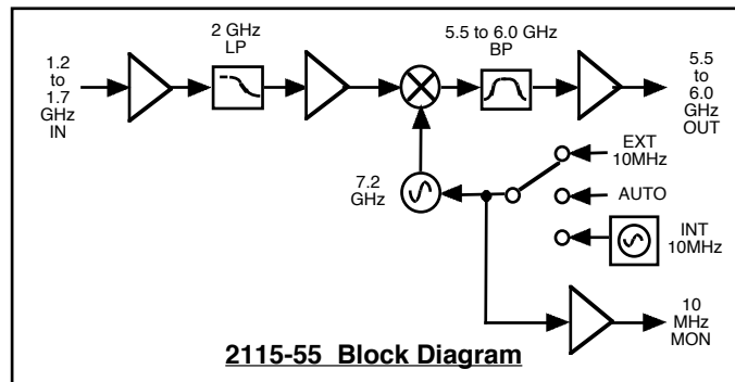
FIGURE 1.2 Model 2115-55 Upconverter Block Diagram
