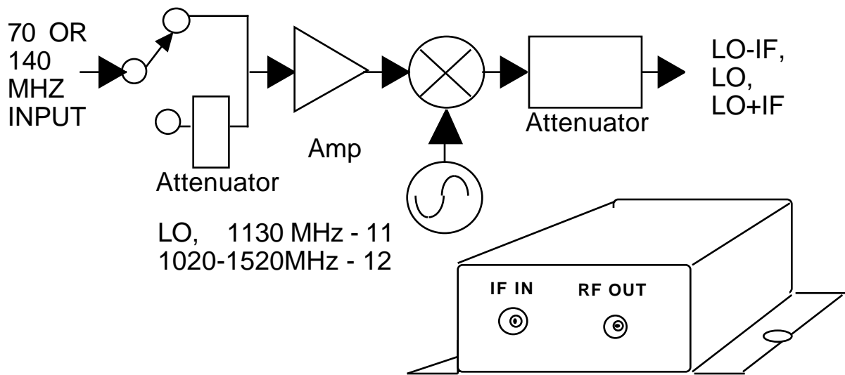
FIGURE 1.1 2006-11, 2006-12 TEST Upconverter Block Diagram and Chassis
