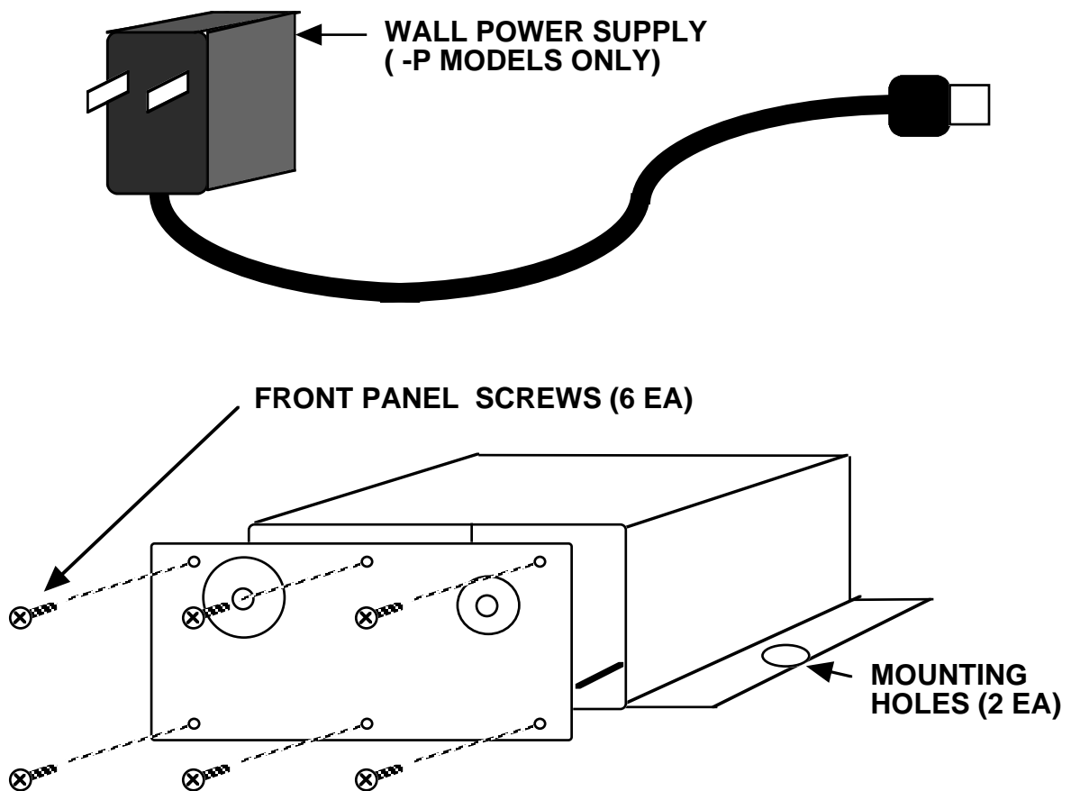
FIGURE 2.1 2006-11, -12 ASSEMBLY DRAWING
