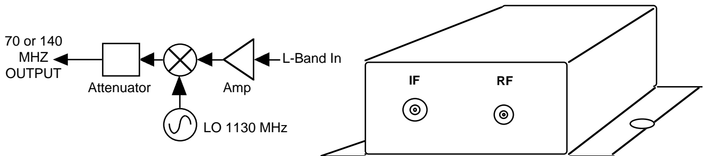
FIGURE 1.1 2006-103 Test Downconverter Block Diagram and Chassis
