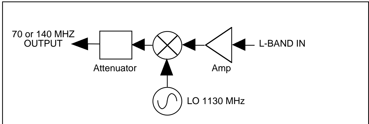
FIGURE 3.1 2006-103 Block Diagram
