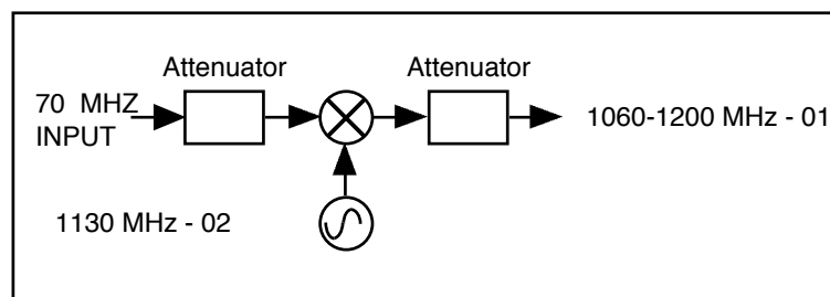
2006-01 Test Upconverter Block Diagram
