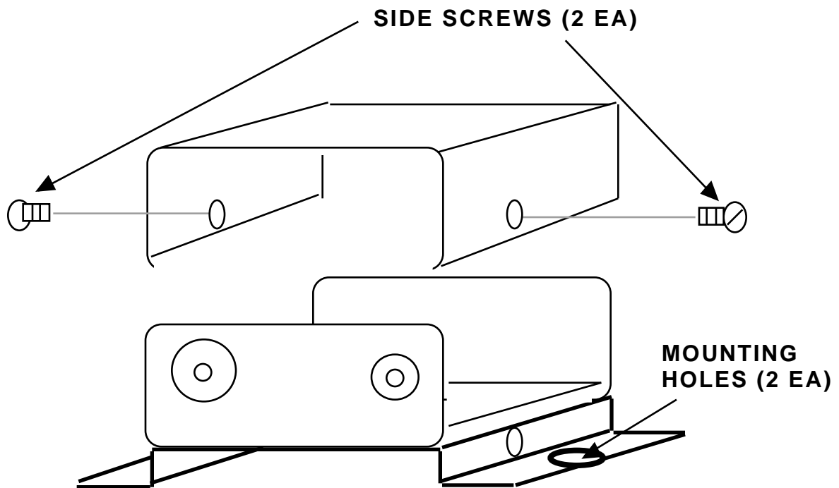
FIGURE 2.1 2006-01 ASSEMBLY DRAWING
