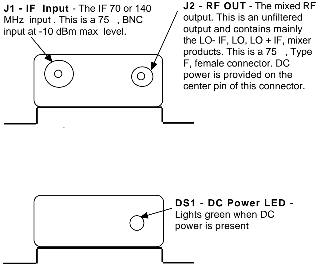
Figure 2.3 2006-01 Input, Output, Power LED
