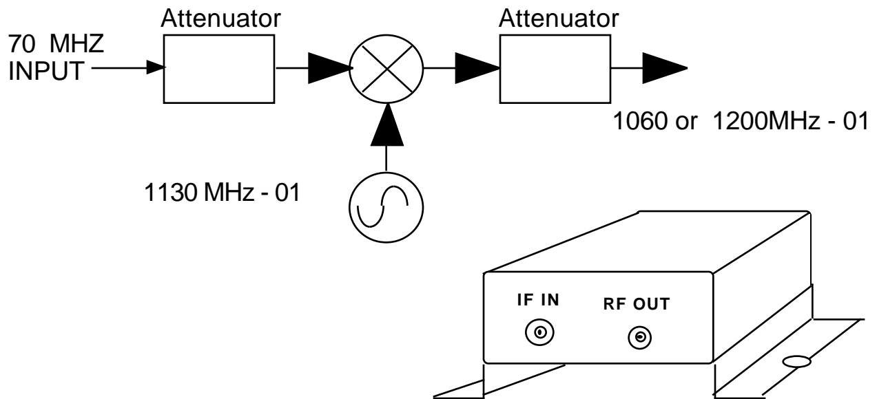
FIGURE 1.1 2006-01 TEST Upconverter Block Diagram and Chassis
