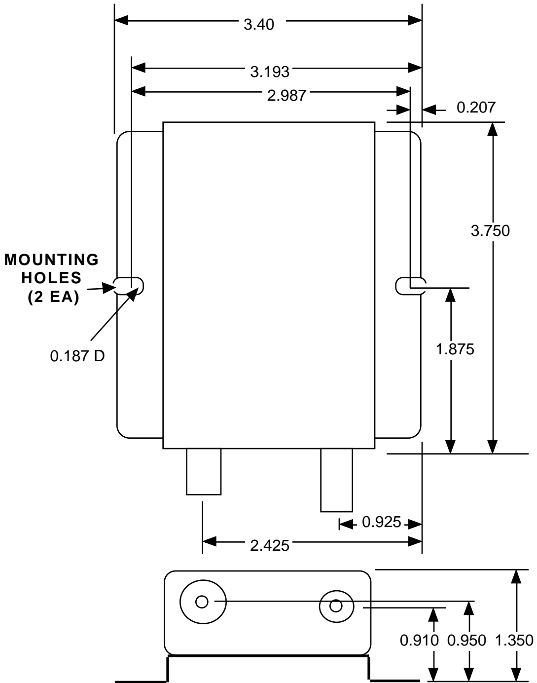
Figure 2.2 2006-01 Package Dimensions
