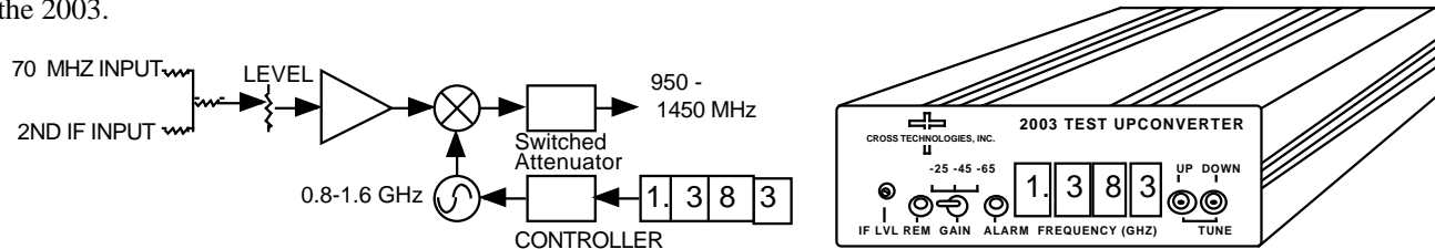
FIGURE 1.1 2003 Agile Test Upconverter Block Diagram and Front Panel
