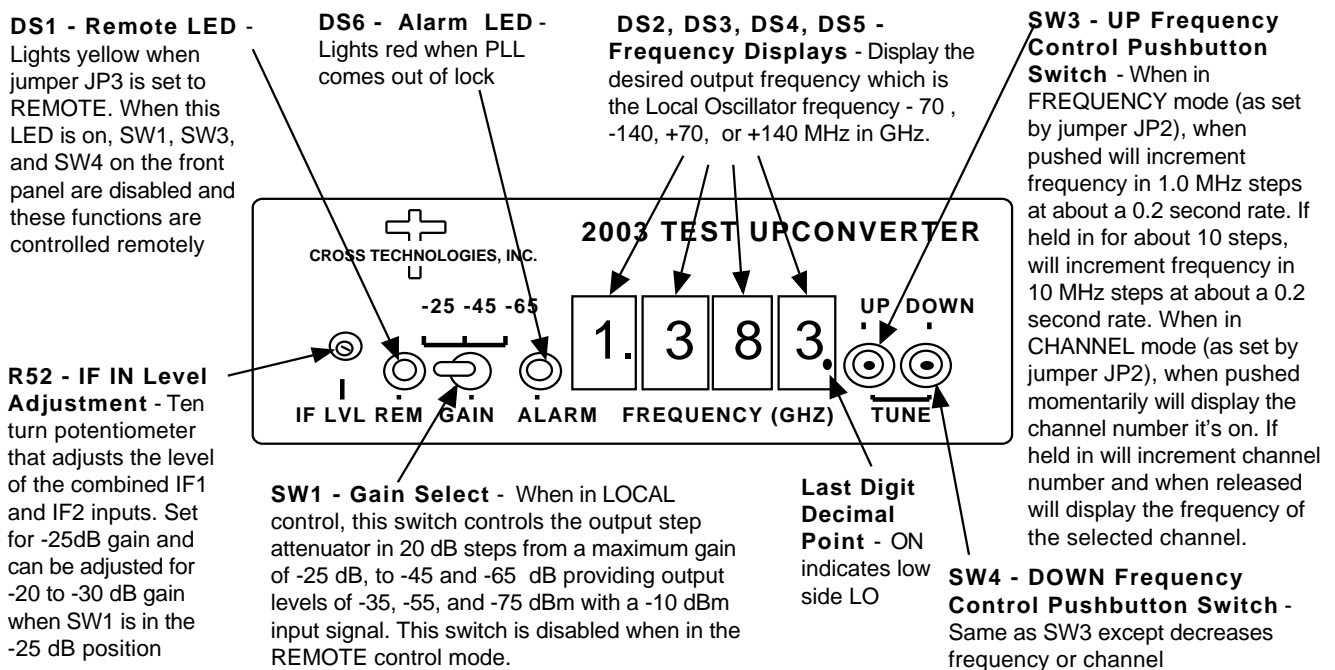
FIGURE 2.2 2003 Front Panel Controls and Indicators
