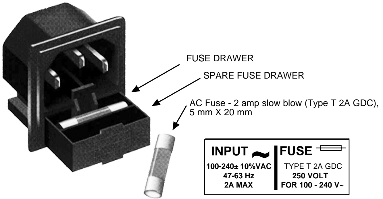
FIGURE 2.7 FUSE LOCATION AND SPARE FUSE
