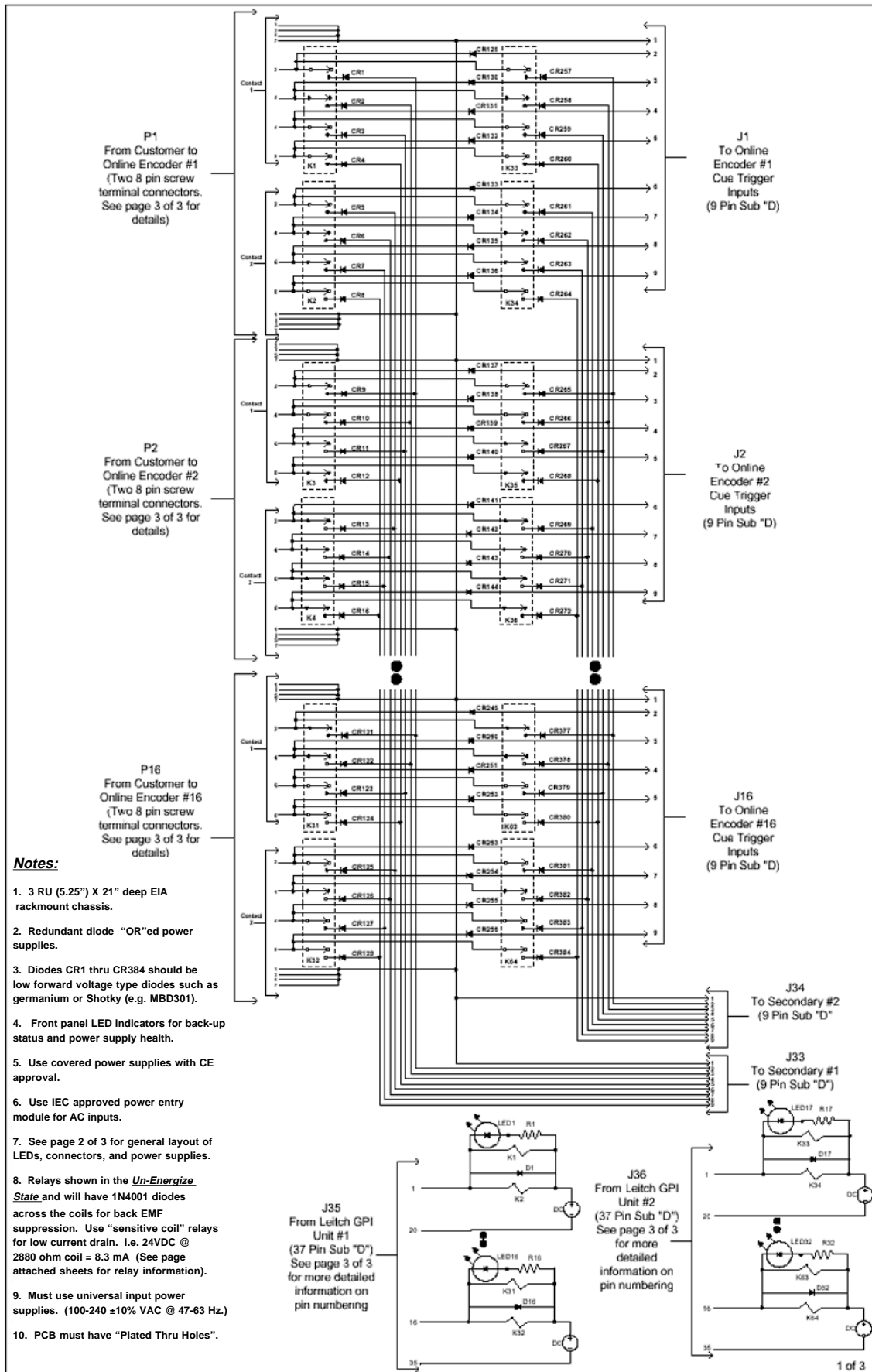
FIGURE 1.3 DETAILED BLOCK DIAGRAM
