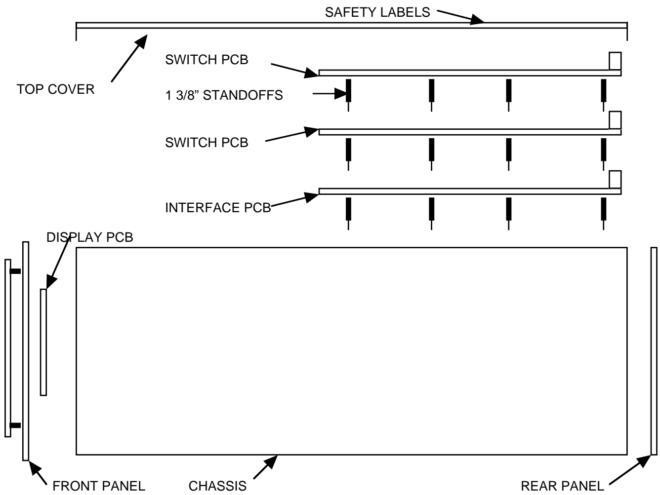
FIGURE 2.0 162 MECHANICAL ASSEMBLY
