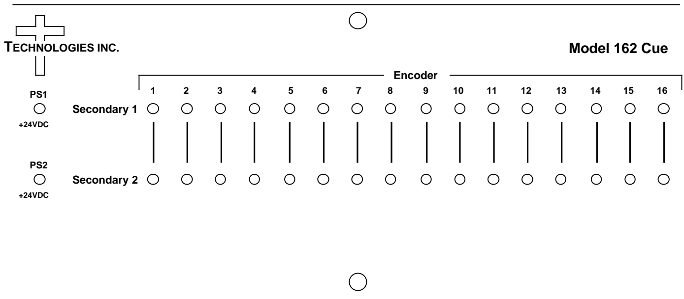
FIGURE 2.5 162 INDICATORS
