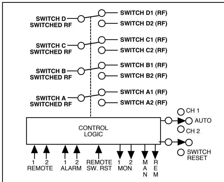
FIGURE 1.2 Model 1582-70L2 RF Switch Block Diagrams
