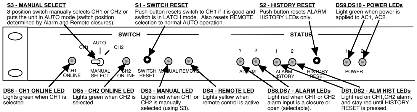
FIGURE 2.3 1582-70L2 Front Panel Controls and Indicators
