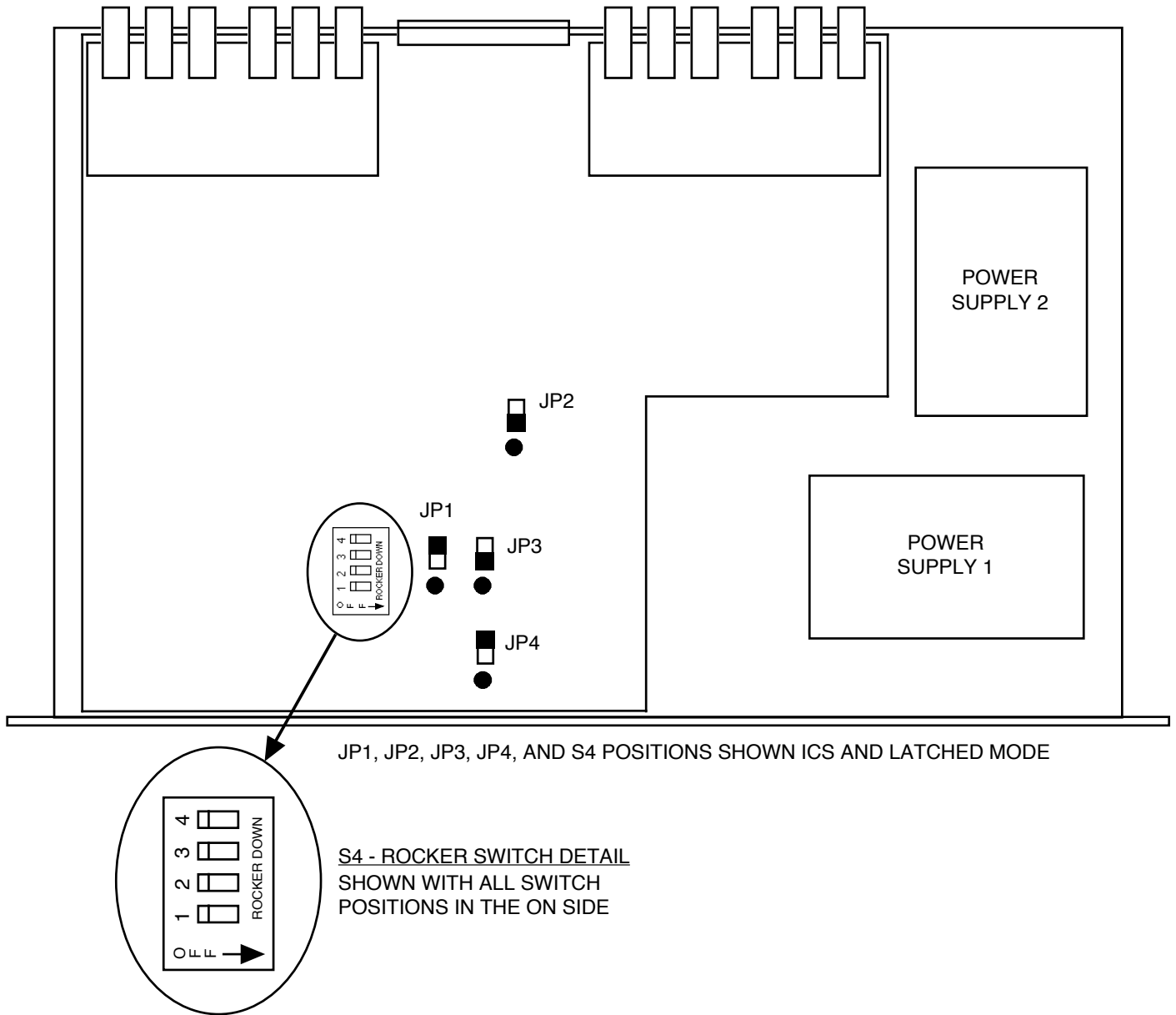
FIGURE 2.1 1582-70L2 RF Switch Assembly
