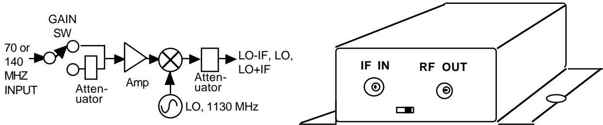
2006-11, -12 Test Upconverter Block Diagram and Chassis
