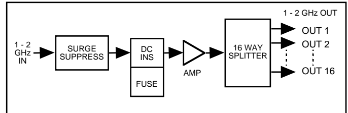
1584-18/18S Block Diagram
