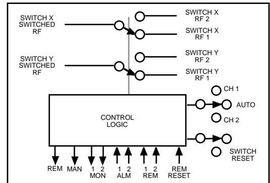
1582-25L BLOCK DIAGRAM
