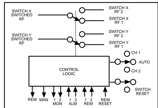
1582-25L BLOCK DIAGRAM
